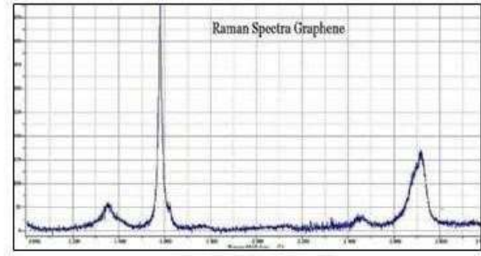
RAMAN Spectrum
